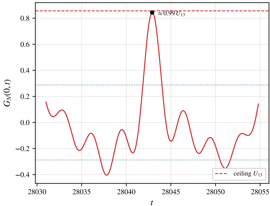
Zoom: the large wave at a near-alignment time
