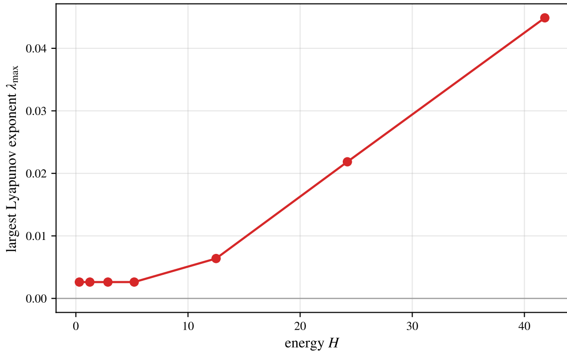
Route to chaos: \lambda_{\max} turns on with energy
