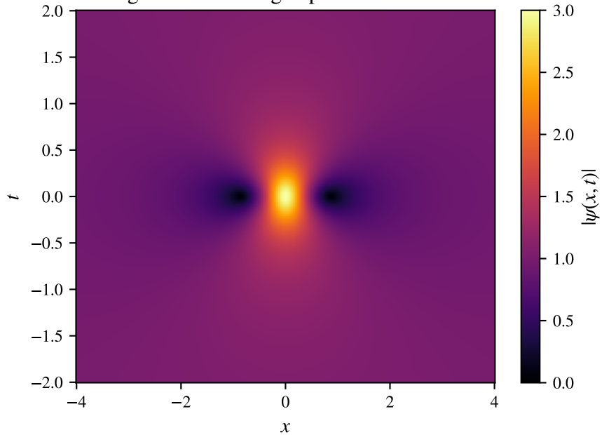
Peregrine soliton: rogue peak from nowhere
