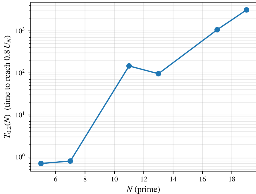
Recurrence time grows exponentially in N
