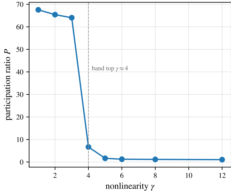
Self-trapping transition
