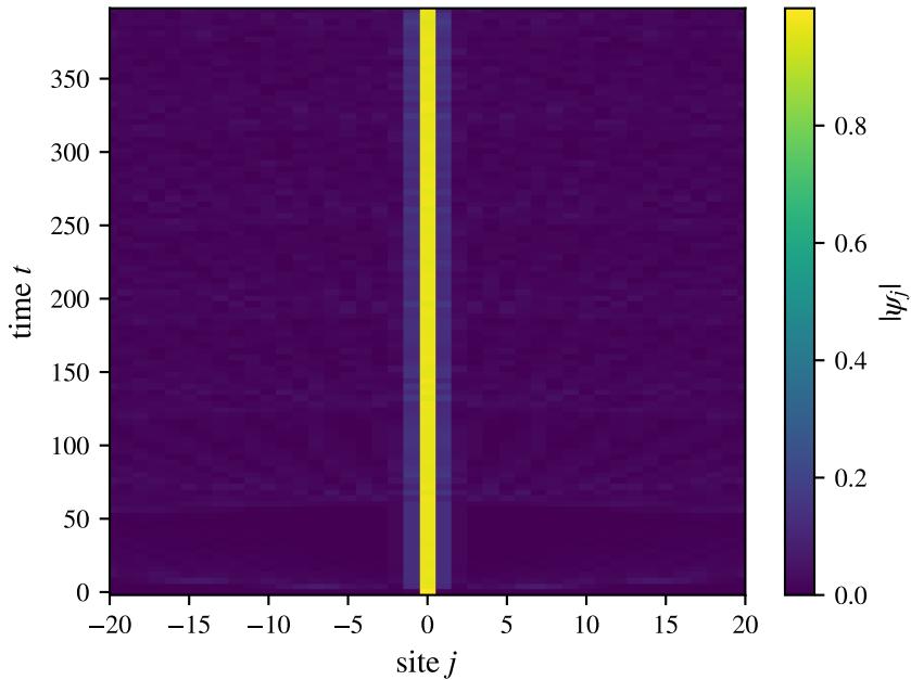
Discrete breather ( \gamma = 8 )
