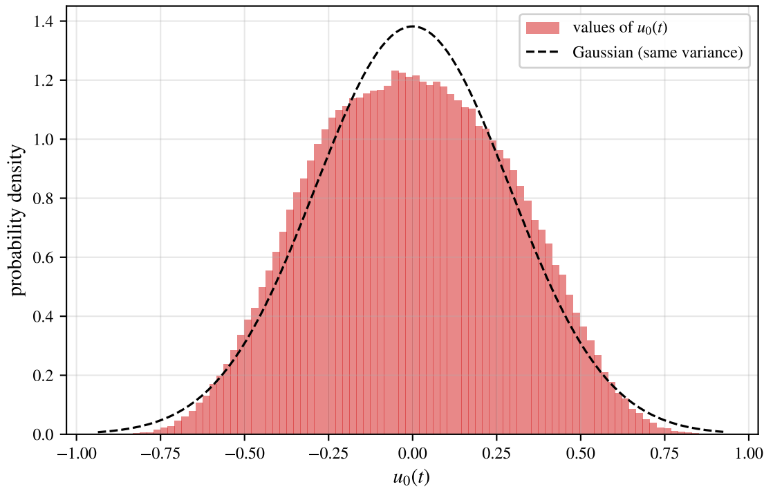
Bohr-Jessen value law: var = 1/12, platykurtic (kurt \approx 2.4 )
