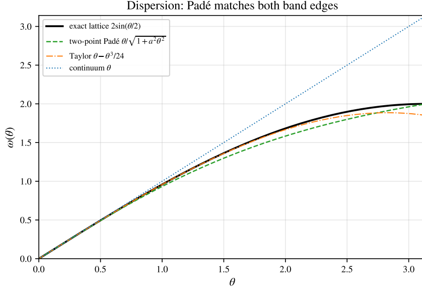
FIGURE 9. Dispersion relations. The exact lattice branch 2 \sin(\theta/2) is matched at both ends by the two-point Padé (22), whereas the continuum \theta and the Taylor truncation \theta - \theta^3/24 diverge at the band edge \theta = \pi ( \bullet , \omega = 2 ).
