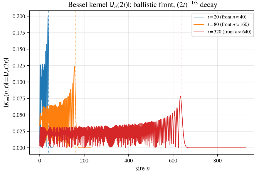
FIGURE 6. Infinite-chain Schrödinger kernel |K_\infty(n, t)| = |J_n(2t)| : a ballistic front at n \approx 2t (dotted) whose height decays as (2t)^{-1/3} . On the ring this kernel is periodized, (19); the effect is intrinsically finite-size.
