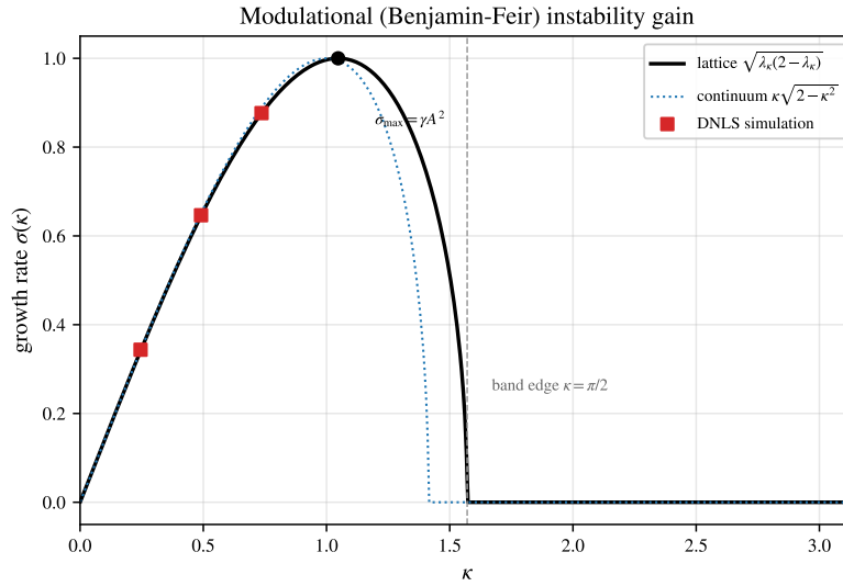
FIGURE 17. Modulational (Benjamin–Feir) instability gain (31) of the plane wave under the DNLS (28): lattice rate (solid), continuum approximation (dotted) and simulated growth rates (squares), with unstable band edge \kappa = \pi/2 and maximal rate \sigma_{\max} = \gamma A^2 .
