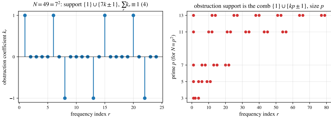
FIGURE 11. The composite obstruction for N = p^2 (Observation 28, exact/gap/prime_square.g). Left: the GAP-computed minimal mod-4 obstruction at N = 49 ( p = 7 )—coefficients \pm 1 on the comb \{1, 6, 8, 13, 15, 20, 22\} = \{1\} \cup \{7k \pm 1\} . Right: the support comb \{1\} \cup \{kp \pm 1\} for p = 3, 5, 7, 11, 13 , of size p .
