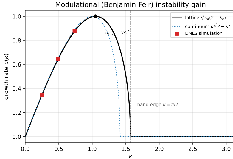
FIGURE 17. Modulational (Benjamin–Feir) instability gain (28) of the plane wave under the DNLS (25): lattice rate (solid), continuum approximation (dotted) and simulated growth rates (squares), with unstable band edge \kappa = \pi/2 and maximal rate \sigma_{\max} = \gamma A^2 .
