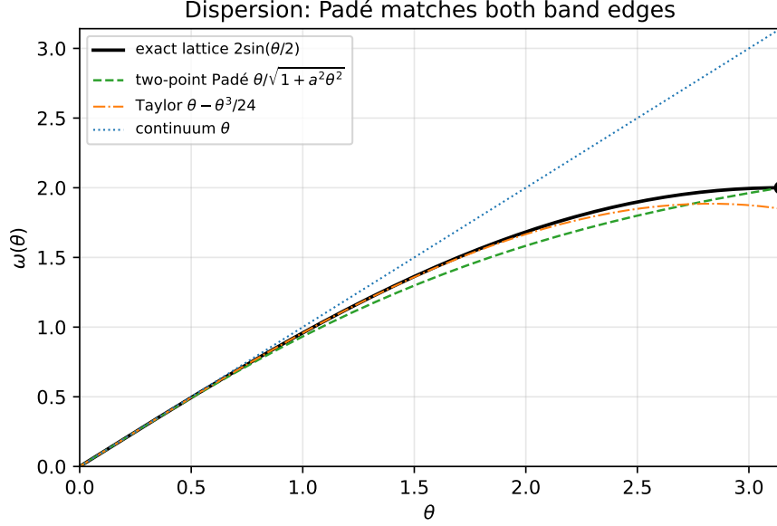
FIGURE 9. Dispersion relations. The exact lattice branch 2\sin(\theta/2) is matched at both ends by the two-point Padé (22), whereas the continuum \theta and the Taylor truncation \theta - \theta^3/24 diverge at the band edge \theta = \pi ( \bullet , \omega = 2 ).
