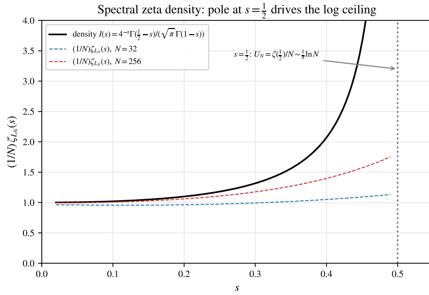
FIGURE 2. The normalized spectral zeta \frac{1}{N} \zeta_{L_N}(s) converges to the symbol density I(s) of (9), which has a pole at s = \frac{1}{2} . The large-wave ceiling is the boundary value U_N = \zeta_{L_N}(\frac{1}{2})/N \sim \frac{1}{\pi} \ln N .
