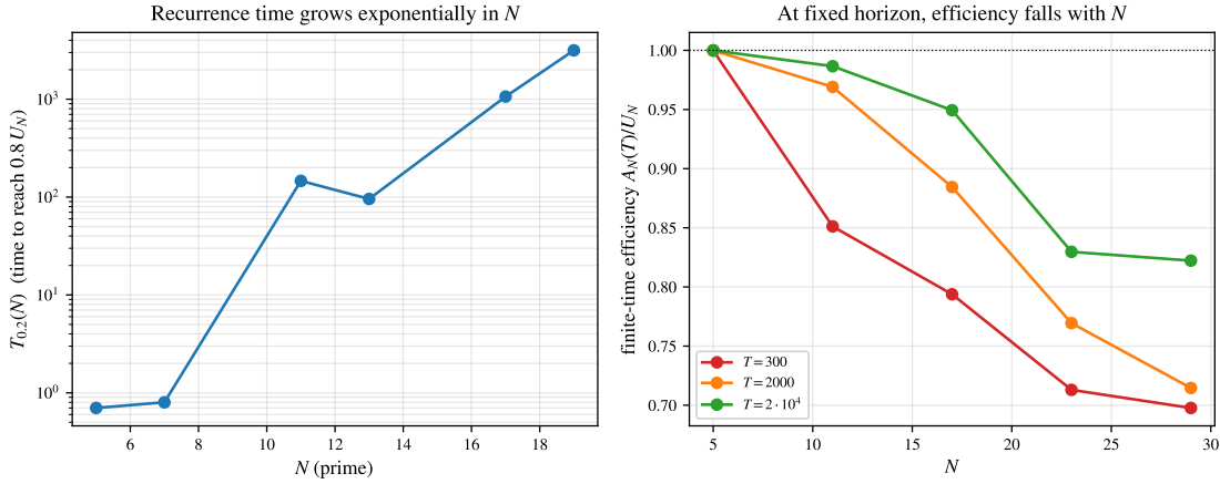
FIGURE 5. Reachability of the ceiling. Left: the recurrence time T_{0.2}(N) to reach 0.8 U_N appears to grow exponentially over the tested prime range (log scale). Right: at a fixed horizon T the finite-time efficiency A_N(T)/U_N decreases with N —more frequencies are harder to align in bounded time. The logarithmic law is an infinite-time ceiling.
