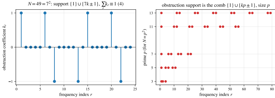
FIGURE 11. The composite obstruction for N = p^2 (Observation 28, exact/gap/prime_square.g). Left: the GAP-computed minimal mod-4 obstruction at N = 49 ( p = 7 )—coefficients \pm 1 on the comb \{1, 6, 8, 13, 15, 20, 22\} = \{1\} \cup \{7k \pm 1\} . Right: the support comb \{1\} \cup \{kp \pm 1\} for p = 3, 5, 7, 11, 13 , of size p .
