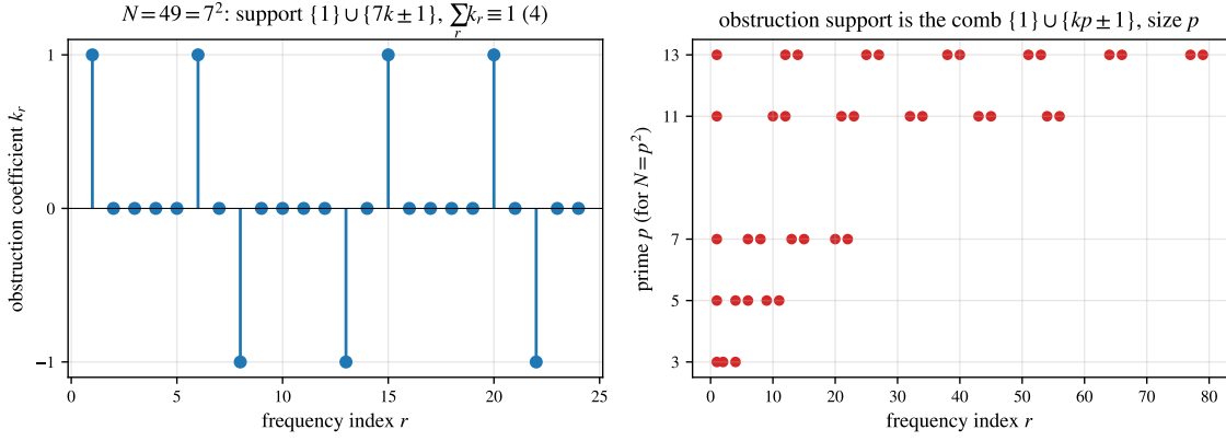
FIGURE 11. The composite obstruction for N = p^2 (Observation 30, exact/gap/prime_square.g). Left: the GAP-computed minimal mod-4 obstruction at N = 49 ( p = 7 )—coefficients \pm 1 on the comb \{1, 6, 8, 13, 15, 20, 22\} = \{1\} \cup \{7k \pm 1\} . Right: the support comb \{1\} \cup \{kp \pm 1\} for p = 3, 5, 7, 11, 13 , of size p .
