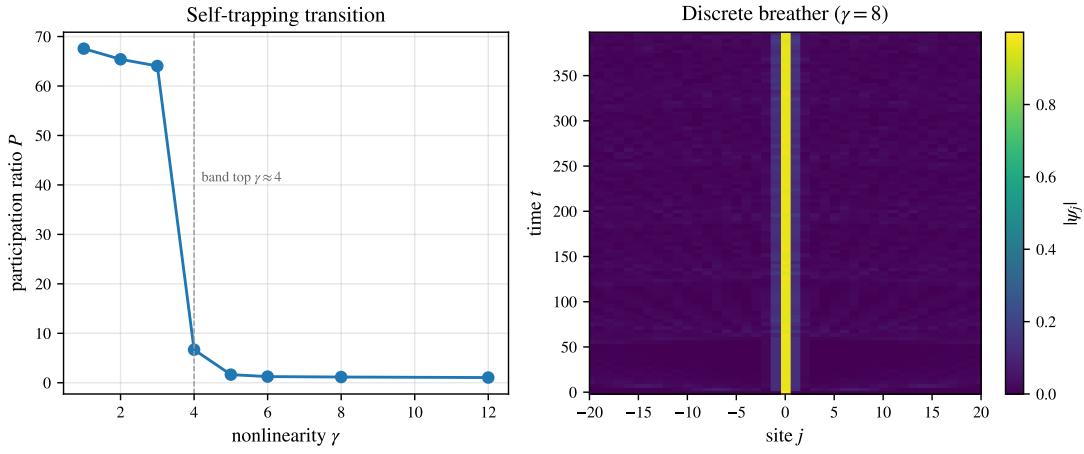
FIGURE 19. DNLS self-trapping ( N = 128 , single-site seed). Left: the participation ratio P collapses from \sim N (dispersed) to \sim 1 (trapped) as the nonlinearity crosses the band top \gamma \approx 4 . Right: above threshold the excitation is a persistent localized breather-like state—a localized column in space-time.
