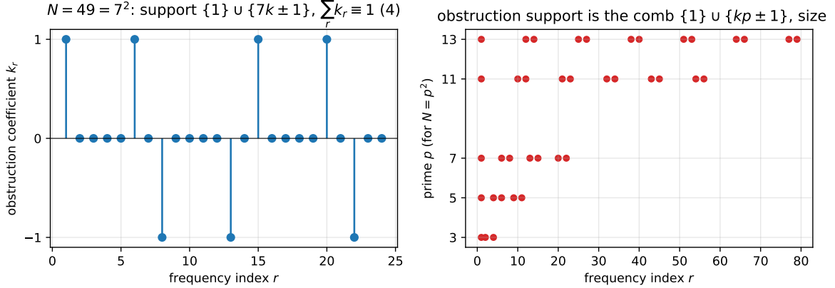
FIGURE 11. The composite obstruction for N = p^2 (Observation 20, exact/gap/prime_square.g ). Left: the GAP-computed minimal mod-4 obstruction at N = 49 ( p = 7 )—coefficients \pm 1 on the comb \{1, 6, 8, 13, 15, 20, 22\} = \{1\} \cup \{7k \pm 1\} . Right: the support comb \{1\} \cup \{kp \pm 1\} for p = 3, 5, 7, 11, 13 , of size p .
