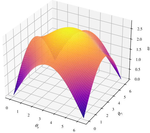
FIGURE 24. Dispersion surface \omega(\theta_x, \theta_y) = 2\sqrt{\sin^2(\theta_x/2) + \sin^2(\theta_y/2)} of the block-circulant Laplacian on the 2-torus: zero at the corners, band top 2\sqrt{2} at the centre.
