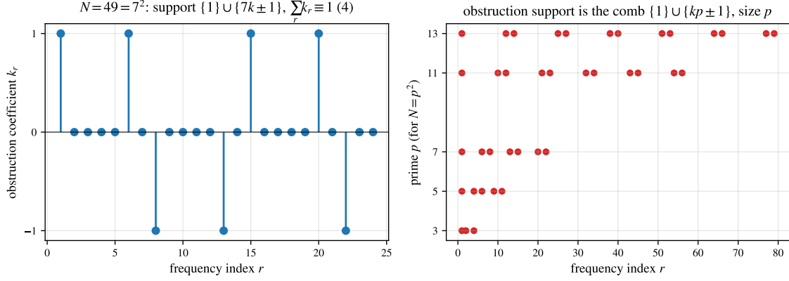
FIGURE 11. The composite obstruction for N = p^2 (Observation 39, exact/gap/prime_square.g). Left: the GAP-computed minimal mod-4 obstruction at N = 49 ( p = 7 )—coefficients \pm 1 on the comb \{1, 6, 8, 13, 15, 20, 22\} = \{1\} \cup \{7k \pm 1\} . Right: the support comb \{1\} \cup \{kp \pm 1\} for p = 3, 5, 7, 11, 13 , of size p .
