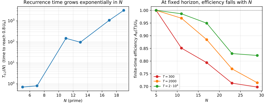
FIGURE 5. Reachability of the ceiling. Left: the recurrence time T_{0.2}(N) to reach 0.8U_N appears to grow exponentially over the tested prime range (log scale). Right: at a fixed horizon T the finite-time efficiency A_N(T)/U_N decreases with N —more frequencies are harder to align in bounded time. The logarithmic law is an infinite-time ceiling.
