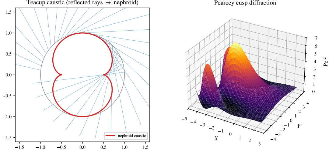
FIGURE 26. The cusp caustic. Left: the everyday teacup caustic—parallel rays reflected inside a circle have a nephroid envelope. Right: the universal Pearcey diffraction |\text{Pe}(X, Y)|^2 of the cusp, bright inside the cusp and dark in the shadow.
