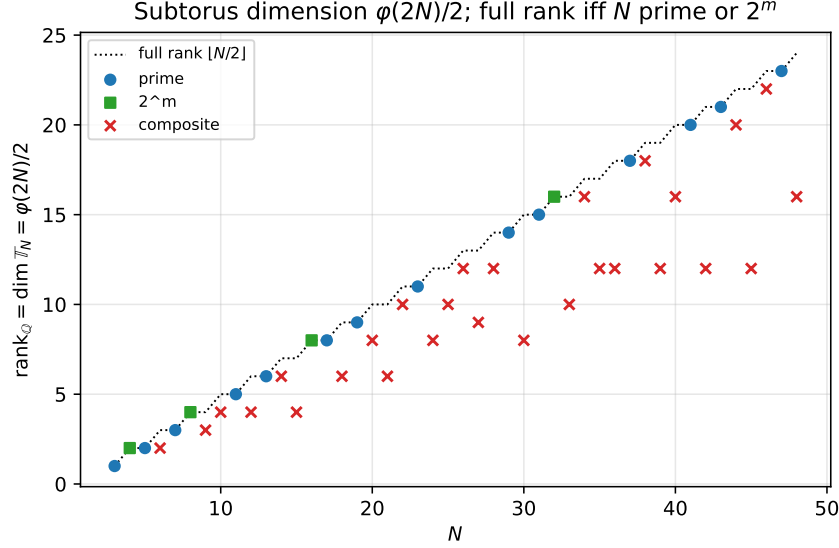
FIGURE 4. The subtorus dimension \frac{1}{2}\phi(2N) (13). Primes and powers of two attain the full rank \lfloor N/2 \rfloor (dotted), so A_N = U_N ; composite N fall below (the sub-torus defect).
