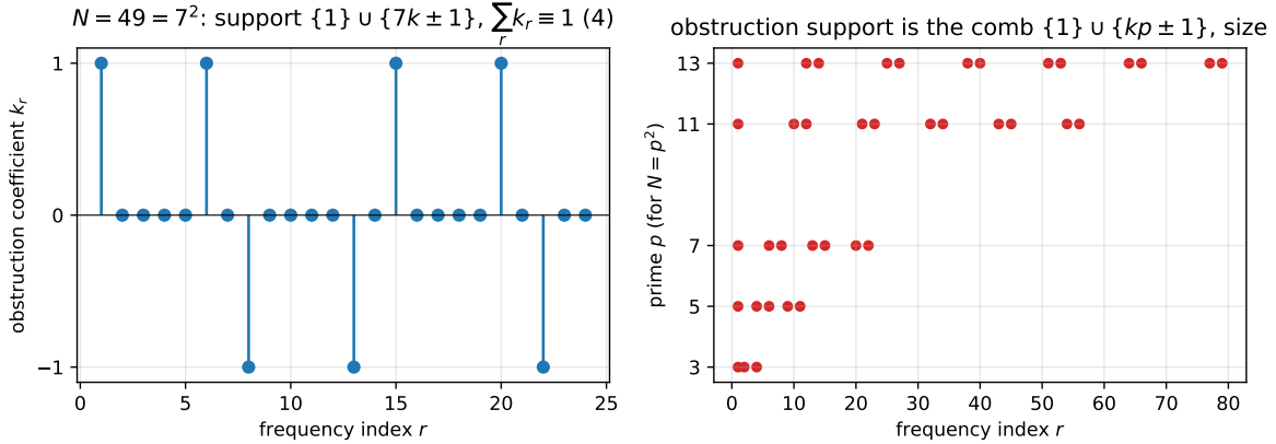
FIGURE 11. The composite obstruction for N = p^2 (Observation 18, exact/gap/prime_square.g ). Left: the GAP-computed minimal mod-4 obstruction at N = 49 ( p = 7 )—coefficients \pm 1 on the comb \{1, 6, 8, 13, 15, 20, 22\} = \{1\} \cup \{7k \pm 1\} . Right: the support comb \{1\} \cup \{kp \pm 1\} for p = 3, 5, 7, 11, 13 , of size p .
