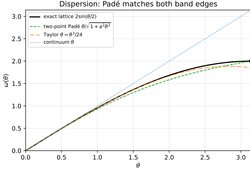
FIGURE 9. Dispersion relations. The exact lattice branch 2 \sin(\theta/2) is matched at both ends by the two-point Padé (21), whereas the continuum \theta and the Taylor truncation \theta - \theta^3/24 diverge at the band edge \theta = \pi ( \bullet , \omega = 2 ).
