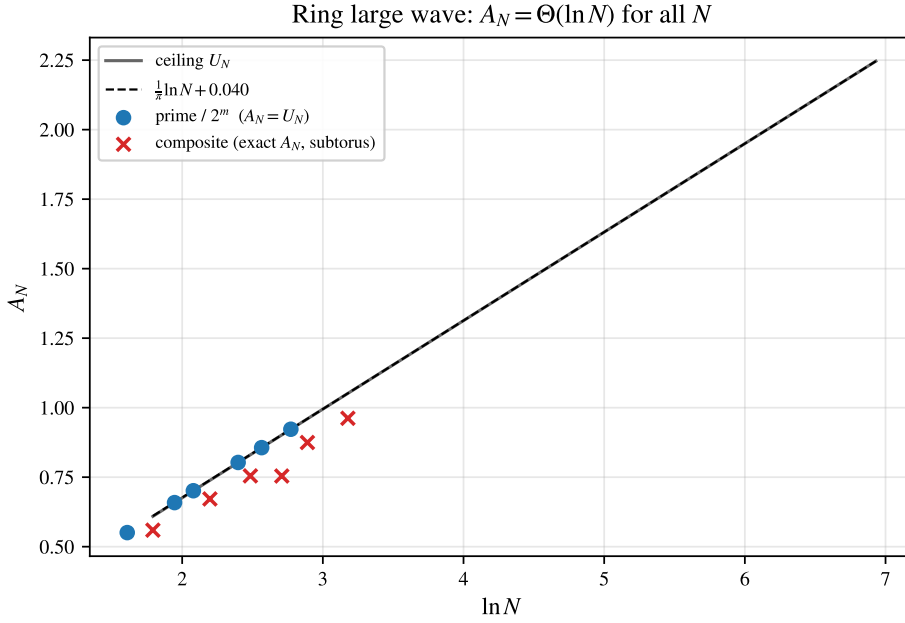
FIGURE 3. Ring large wave A_N versus \ln N . The ceiling U_N (Lemma 2) grows as \frac{1}{\pi} \ln N + 0.040 ; for primes and N = 2^m the supremum equals U_N (Theorems 3, 4); for composite N the (numerically evaluated) subtorus value lies slightly below, and A_N \sim \frac{1}{\pi} \ln N for every N (Theorem 6).
