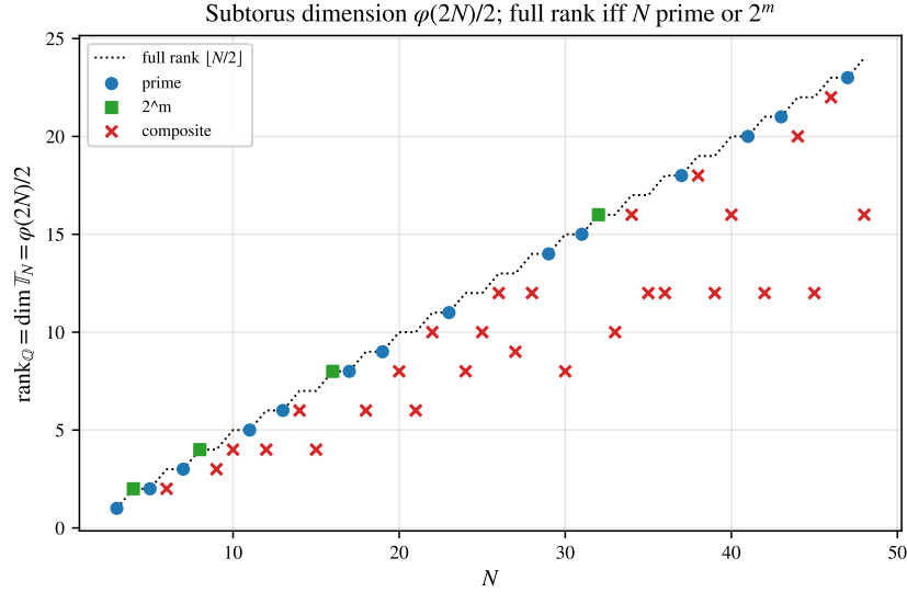
FIGURE 4. The subtorus dimension \frac{1}{2}\varphi(2N) (13). Primes and powers of two attain the full rank \lfloor N/2 \rfloor (dotted), so A_N = U_N ; composite N fall below (the sub-torus defect).
