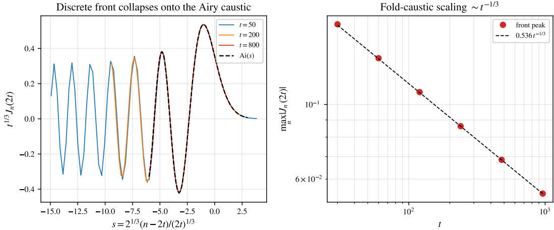
FIGURE 28. The discrete-Schrödinger front as a fold caustic. Left: the rescaled fronts t^{1/3} J_n(2t) for t = 50, 200, 800 collapse onto the Airy function \text{Ai}(s) , s = 2^{1/3}(n - 2t)/(2t)^{1/3} (Eq. (38)). Right: the front peak follows the universal fold scaling 0.536 t^{-1/3} .
