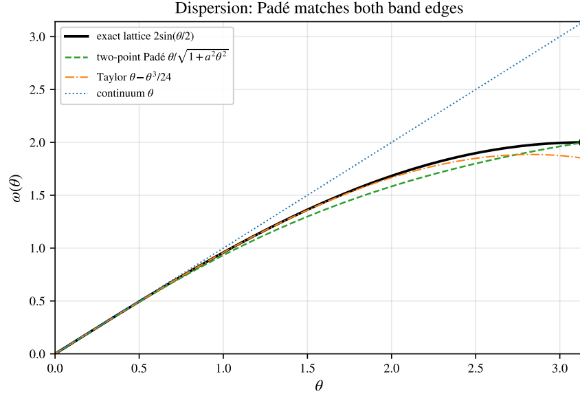
FIGURE 9. Dispersion relations. The exact lattice branch 2 \sin(\theta/2) is matched at both ends by the two-point Padé (27), whereas the continuum \theta and the Taylor truncation \theta - \theta^3/24 diverge at the band edge \theta = \pi ( \bullet , \omega = 2 ).
