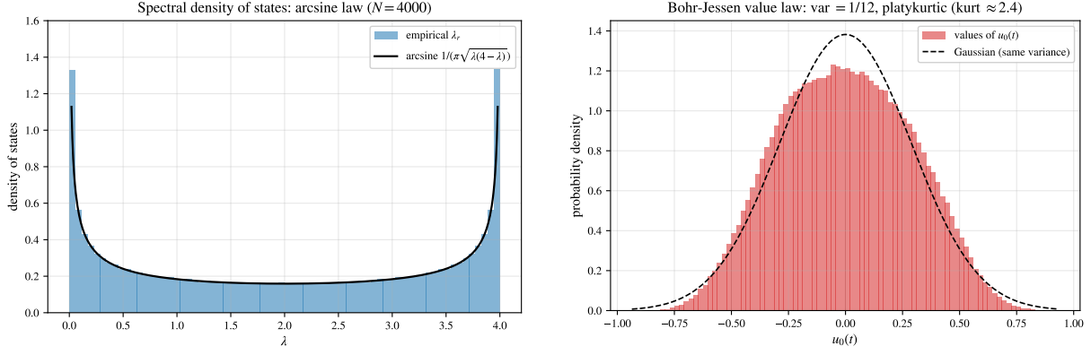
FIGURE 13. Left: spectral density of states converges to the arcsine law (28). Right: the Bohr–Jessen value law of u_0(t) —symmetric, variance (N^2 - 1)/(12N^2) \rightarrow 1/12 , platykurtic (flatter than the Gaussian of equal variance, dashed).
