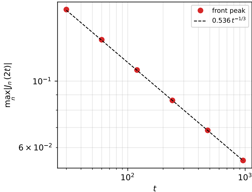
Fold-caustic scaling \sim t^{-1/3}
