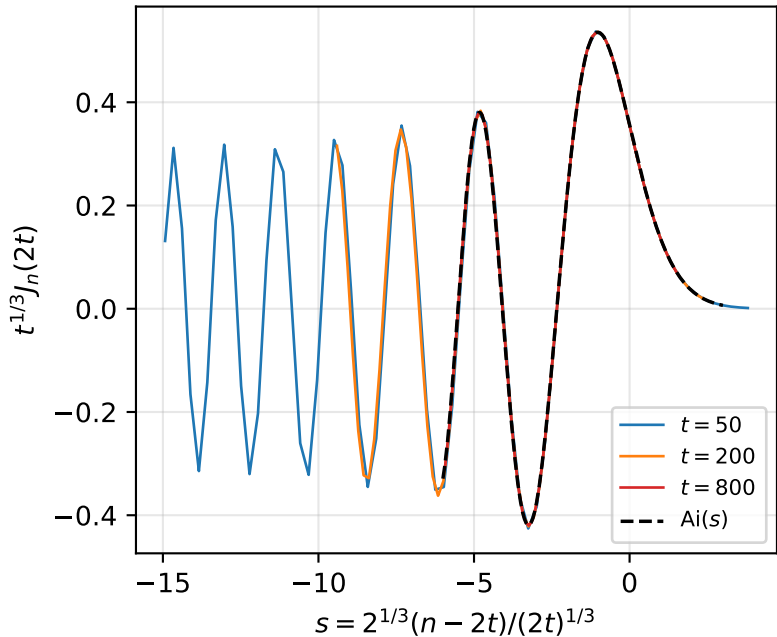
Discrete front collapses onto the Airy caustic
