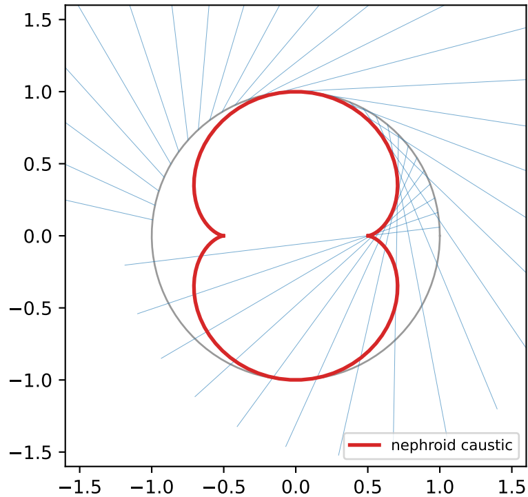
Teacup caustic (reflected rays \rightarrow nephroid)
