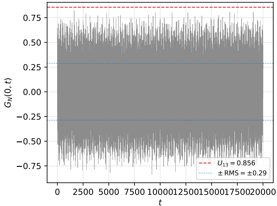
Thin-tailed bulk with rare spikes ( N = 13 )
