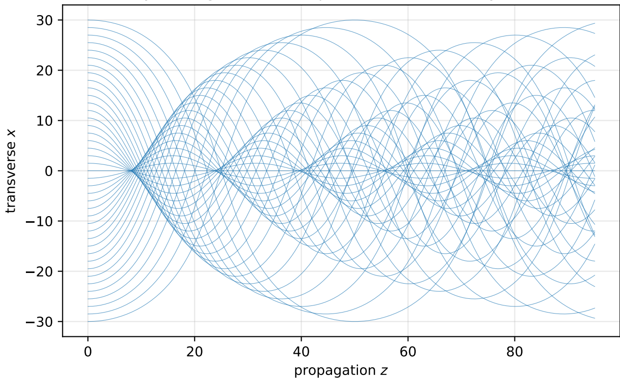
Ray tracing in a current jet: caustic from a ray bundle
