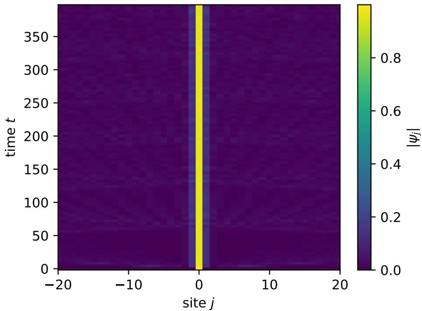
Discrete breather ( \gamma = 8 )
