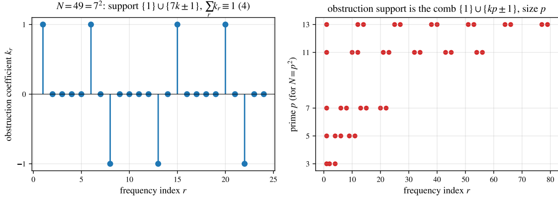
FIGURE 11. The composite obstruction for N = p^2 (Observation 34, exact/gap/prime_square.g ). Left: the GAP-computed minimal mod-4 obstruction at N = 49 ( p = 7 )—coefficients \pm 1 on the comb \{1, 6, 8, 13, 15, 20, 22\} = \{1\} \cup \{7k \pm 1\} . Right: the support comb \{1\} \cup \{kp \pm 1\} for p = 3, 5, 7, 11, 13 , of size p .
