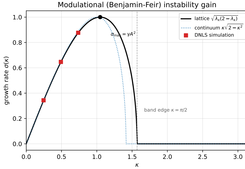
FIGURE 17. Modulational (Benjamin–Feir) instability gain (27) of the plane wave under the DNLS (24): lattice rate (solid), continuum approximation (dotted) and simulated growth rates (squares), with unstable band edge \kappa = \pi/2 and maximal rate \sigma_{\max} = \gamma A^2 .
