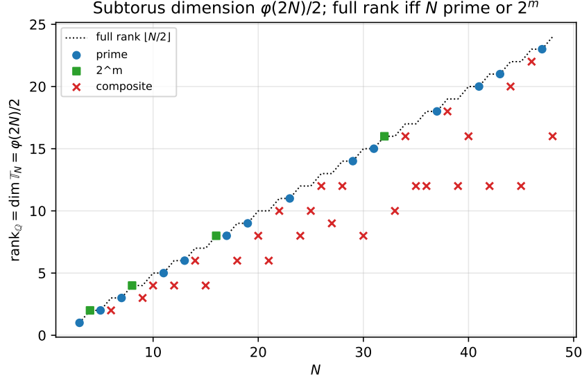
FIGURE 4. The subtorus dimension \frac{1}{2}\phi(2N) (13). Primes and powers of two attain the full rank \lfloor N/2 \rfloor (dotted), so A_N = U_N ; composite N fall below (the sub-torus defect).
