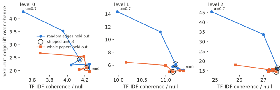
Figure 1. The structure/meaning trade-off across \alpha : held-out hyperedge lift against TF-IDF coherence over its null, holding out random edges (blue) or whole papers (orange). The ring marks \alpha = 0.3 .
