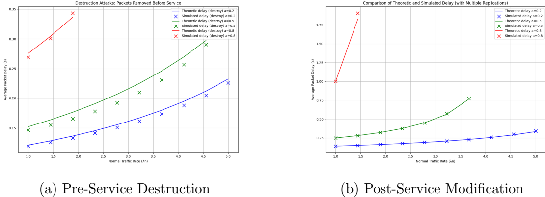
Figure 2: Single-node delay comparison. Note how modification attacks cause a much faster escalation in delay due to the server resources wasted on corrupted packets.
