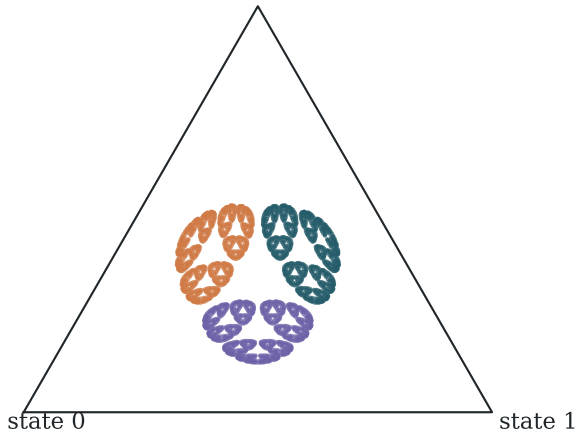
Beliefs B_7
