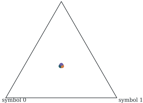
Next-token vectors
