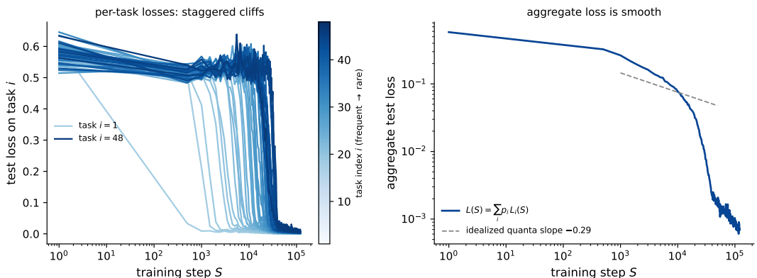
Figure 8: Multitask sparse parity [57]: smooth scaling from staggered cliffs. Setup: T = 48 subtasks with Zipfian frequencies p_i \propto i^{-(\alpha+1)} , \alpha = 0.4 ; inputs are a one-hot task indicator ( T bits) concatenated with 24 random \pm 1 bits; the label is the parity of a fixed random 3-subset of the bits, the subset depending on the task. Model: one-hidden-layer ReLU MLP, width 512, MSE loss on \pm 1 labels, trained online (fresh batches of 256; Adam, learning rate 2 \times 10^{-3} , 1.2 \times 10^5 steps; fixed seed). Left : test loss per subtask vs. training step. Each subtask is learned in an abrupt cliff, frequent tasks first. Right : the frequency-weighted aggregate L(S) = \sum_i p_i L_i(S) is smooth; the dashed guide is the idealized quanta-model slope -\alpha/(\alpha+1) from Exercise 7.1(d). The measured decay is visibly steeper, as discussed in the text.
