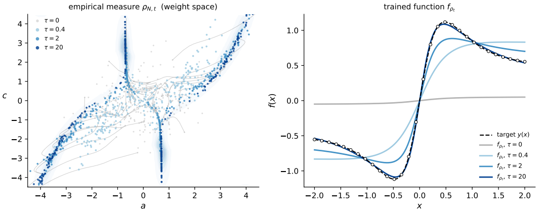
Figure 6: Mean-field training for a d = 1 example: f_{\rho}(x) = \frac{1}{N} \sum_i c_i \tanh(a_i x) , trained by the rescaled gradient flow (5.15) on n = 30 samples of the two-neuron teacher y(x) = 2 \tanh(3x) - \frac{3}{2} \tanh(x) ; \tau = \tilde{\eta} t is rescaled training time. Left : the empirical measure \rho_{N,t} in the (a, c) plane for N = 300 (dots, colored by time; thin gray lines trace 40 of the particle trajectories), drawn over the density of an N = 30,000 run at \tau = 20 (shaded contours), standing in for the limiting measure \rho_t . Individual neurons move order-one distances, and the measure condenses onto one-dimensional filaments — the configurations realizing the teacher. (The point symmetry (a, c) \mapsto (-a, -c) reflects the oddness of \tanh .) Right : the mean field itself, f_{\rho_t}(x) , converging to the target (dashed; circles mark the training data).
