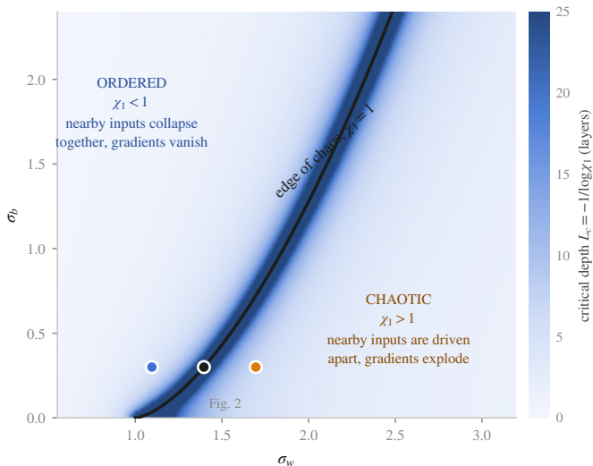
Figure 5: Order/chaos phase diagram for a tanh network, with shading indicating the critical depth to which a network is trainable.
