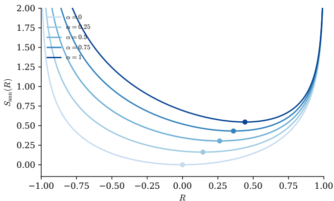
Figure 9: The annealed action S_{\text{ann}}(R) of the spherical perceptron, (A.8), for \alpha \in \{0, 0.25, 0.5, 0.75, 1\} (bottom to top at R = 0 ), with the minimizer marked on each curve. The entropy pins the minimum at R = 0 when \alpha = 0 ; increasing the load slides it smoothly toward larger overlap, and the entropic wall at R = 1 keeps it in the interior. One basin at every \alpha , moving continuously: no phase transition.
