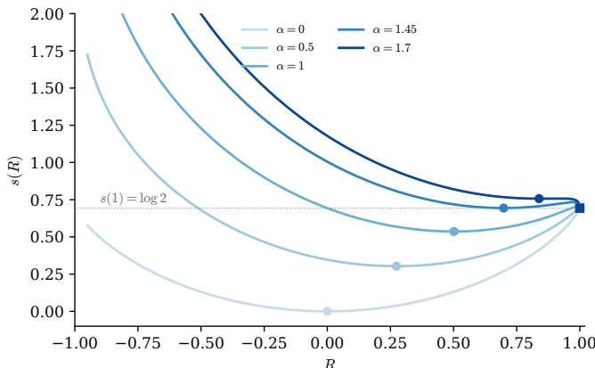
Figure 15: The annealed action s(R) of the Ising perceptron, (2.44), for several loads. Interior local minima are marked with circles; the teacher state R = 1 , where s(1) = \log 2 exactly, with squares. The two basins exchange dominance near \alpha \approx 1.45 .
