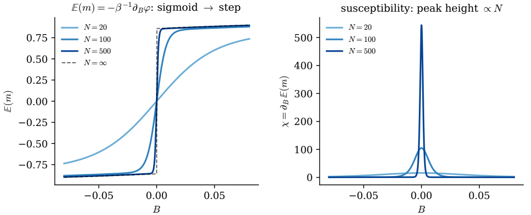
Figure 3: Fingerprints of a first-order transition, in the mean-field Ising model at \beta dJ = 1.5 , computed from the one-dimensional integral (2.25) at finite N . Left: the expected magnetization as a function of the field is a sigmoid of width \propto 1/N , sharpening into a step. Right: the susceptibility \chi = \partial_B E(m) is a peak of height \propto N and width \propto 1/N .
