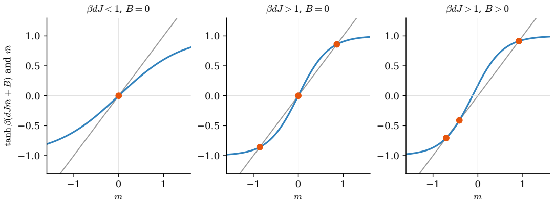
Figure 1: Graphical solution of the mean-field equation (2.27): intersections of \tanh \beta(dJ\bar{m} + B) with the diagonal. Left: high temperature, one solution at \bar{m} = 0 . Middle: low temperature at B = 0 , three solutions, of which \bar{m} = 0 is a maximum of s and \pm\bar{m} are degenerate minima. Right: low temperature with B > 0 , three solutions, with the positive one the global minimum.
