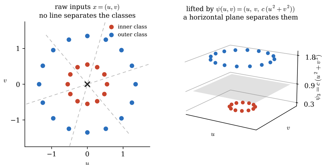
Figure 12: One fixed extra feature can make a hard problem linear. Left: two classes of points in the plane, on concentric rings. No line separates them, since the convex hull of each class contains the origin. Right: after appending the single feature \psi_3 = c(u^2 + v^2) , the rings sit at two different heights, and a horizontal plane \psi_3 = cr_0^2 separates them. Nothing has been learned: we supplied the radial coordinate.
