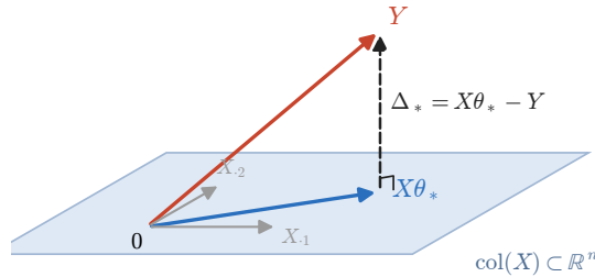
Figure 10: Least squares, geometrically. The normal equations X^T \Delta_* = 0 say that the residual is orthogonal to the column space of X , so the fitted prediction vector X\theta_* is the orthogonal projection of Y onto \text{col}(X) . “Orthogonal” refers to the Euclidean metric \delta_{\mu\nu} on the space \mathbb{R}^n of function values on the training set.
