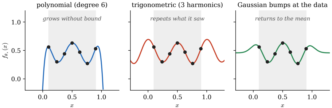
Figure 11: Choosing \psi is choosing the model. The same seven data points (black), interpolated exactly by three different fixed feature maps with P = n = 7 : polynomials of degree six, trigonometric functions of period one with three harmonics, and Gaussian bumps centered at the data. All three drive the training loss to zero; they disagree everywhere outside the training range (shaded), and that disagreement was decided before the labels were read.
