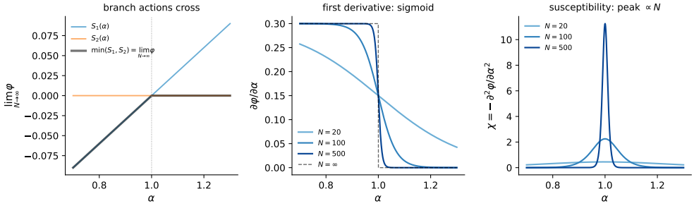
Figure 14: Anatomy of a first-order transition at finite N , in the minimal two-branch model \varphi_1(B) = 0.3(B - B_c) , \varphi_2 \equiv 0 , with the control parameter written as \alpha . Left: the branch free energies cross at B_c ; the limiting free-energy density is their minimum, which has a kink. Middle: at finite N , \partial_B \varphi is the probability-weighted average of the branch slopes (2.36), a sigmoid of width \propto 1/N . Right: the susceptibility (2.37) peaks at B_c with height \propto N and width \propto 1/N .
