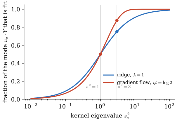
Figure 13: Ridge regression and early-stopped gradient flow as spectral filters: the fraction of a data mode u_a \cdot Y that is fit, as a function of the mode's kernel eigenvalue s_a^2 . The two are tuned to agree on the mode with s^2 = 1 , and disagree elsewhere; the dots mark the two-mode example of Exercise B.5.
