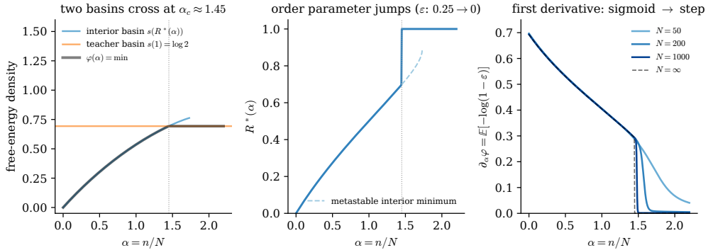
Figure 16: The Ising perceptron’s phase transition. Left: the free-energy densities of the interior basin, s(R^*(\alpha)) , and of the teacher basin, s(1) = \log 2 , cross at \alpha_c \approx 1.45 ; the limiting \varphi(\alpha) is their minimum, with a kink. Middle: the order parameter R^*(\alpha) jumps from 0.70 to 1; the dashed continuation is the metastable interior minimum, which disappears at the spinodal \alpha \approx 1.73 . Right: at finite N , \partial_\alpha \varphi = \mathbb{E}[-\log(1 - \varepsilon)] , computed from the integral (2.44), is a sigmoid sharpening into the step of height \approx 0.29 .
