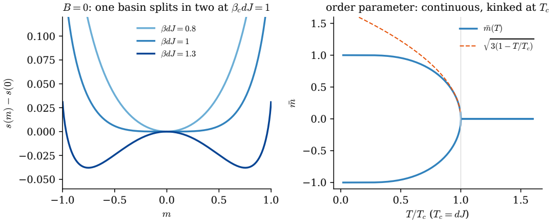
Figure 4: The second-order transition of the mean-field Ising model at B = 0 . Left: the action s(m) for temperatures above, at, and below T_c = dJ ; a single basin flattens and splits into two symmetric ones. Right: the resulting magnetization \bar{m}(T) , continuous at T_c but with the square-root singularity (2.32) (dashed).
