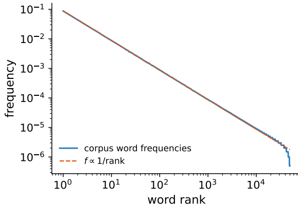
Figure 7: Zipf’s law, illustrated on a synthetic corpus: 2 \times 10^6 tokens drawn from a 1/k distribution over a vocabulary of 5 \times 10^4 words, with the empirical rank–frequency curve against the f \propto 1/\text{rank} guide. The curve is a consistency check rather than data, since the words were sampled from a Zipf distribution to begin with. Real corpora look the same over roughly four decades, with deviations at both ends: the Zipf–Mandelbrot correction at low rank, and a steeper tail beyond about 10^4 words.
