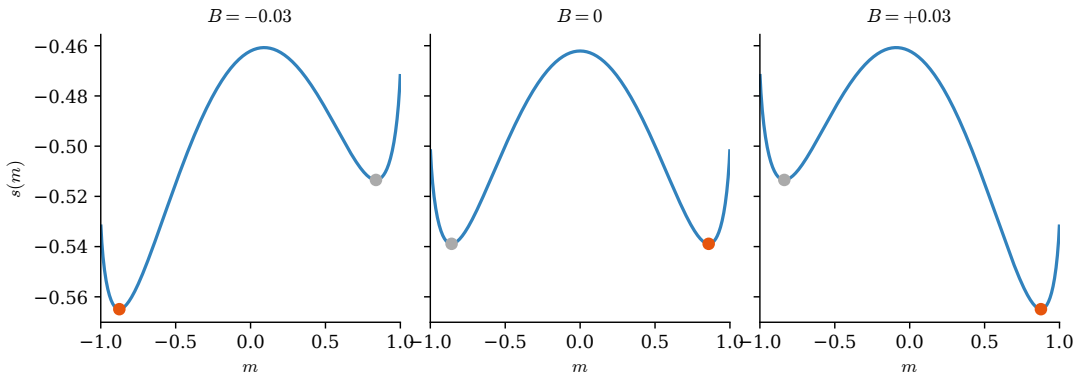
Figure 2: The action s(m) of (2.25) in the ordered phase ( \beta dJ = 1.5 ), for a negative, zero, and positive external field. The two minima tilt with B ; the global minimum (orange) switches sides at B = 0 . The suppressed minimum (grey) survives as a metastable state.
