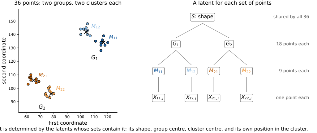
Figure 1: One draw from the finite model. The left panel shows the 36 points; the right panel shows which set of observations receives each parameter. The global shape S is available to every observation.
