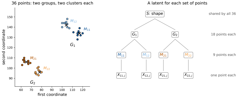
Each point is determined by the latents whose sets contain it: its shape, group centre, cluster centre, and its own position in the cluster.
