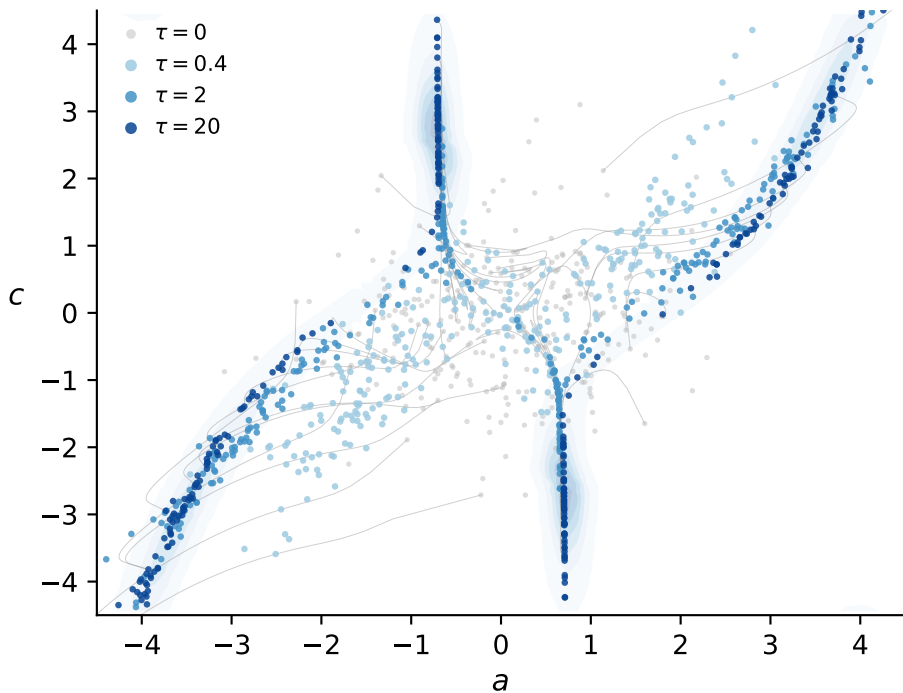
empirical measure \rho_{N,t} (weight space)
