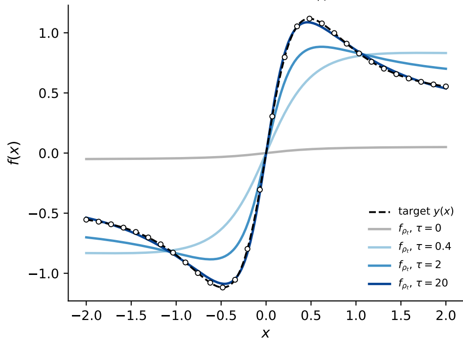
trained function f_{\rho_t}
