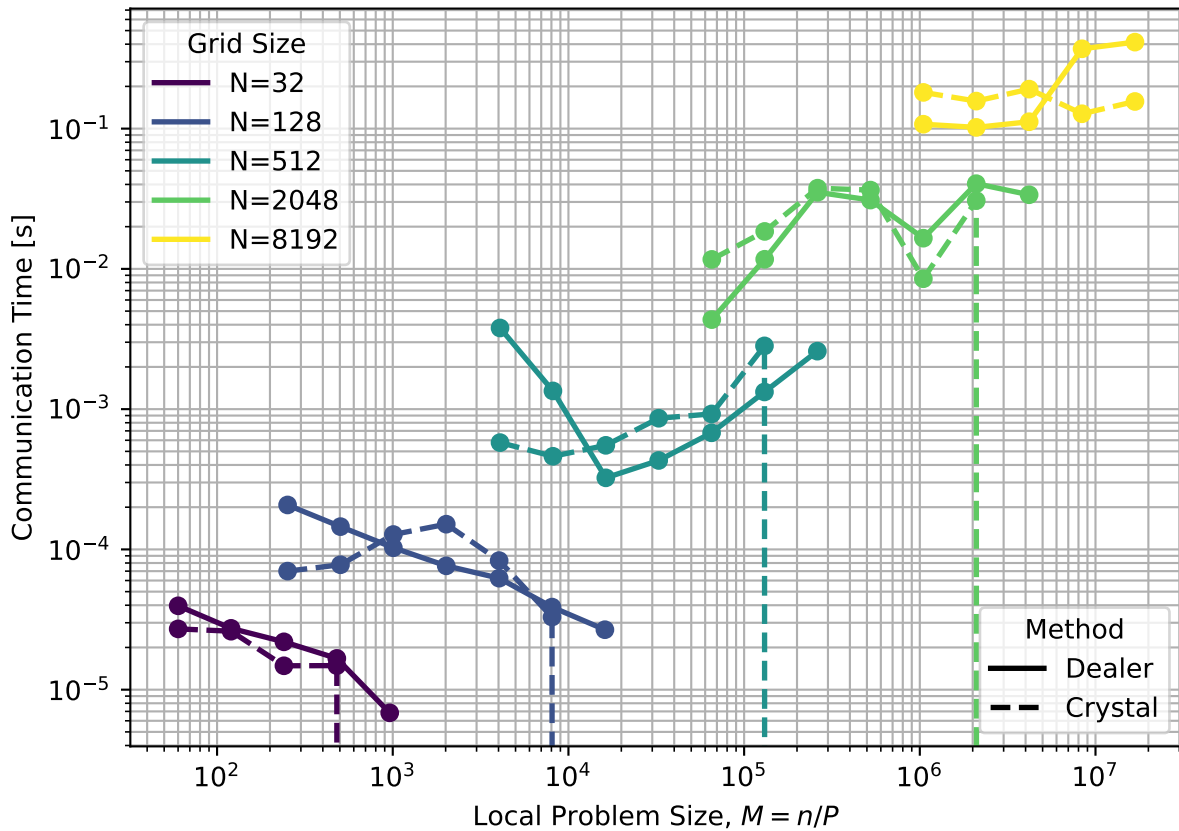
Communication Time vs Local Problem Size
