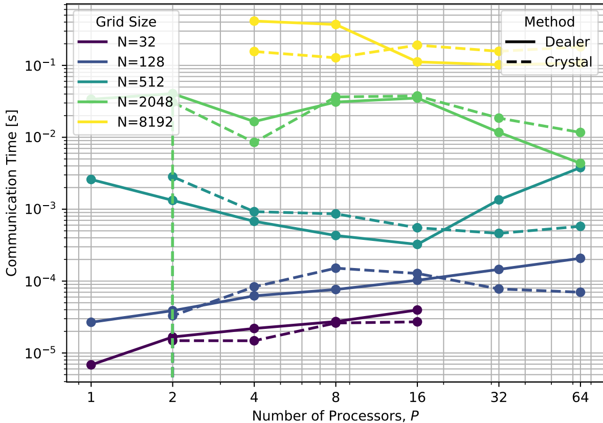
Communication Time vs Processor Count
