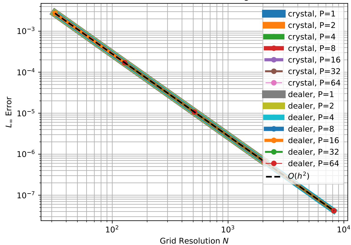
Poisson Solver Grid Convergence
