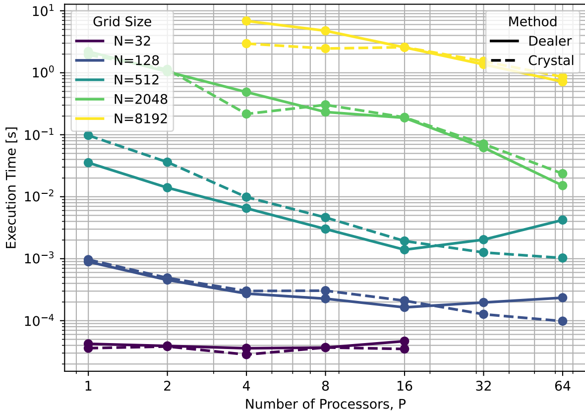
Poisson Solver Execution Time
