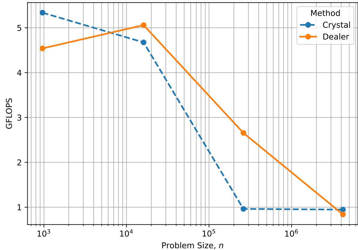
Single-Processor Poisson Solver Performance
