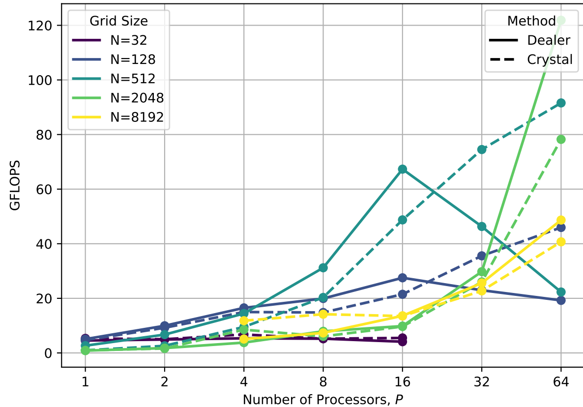
Poisson Solver Performance (GFLOPS vs P)
