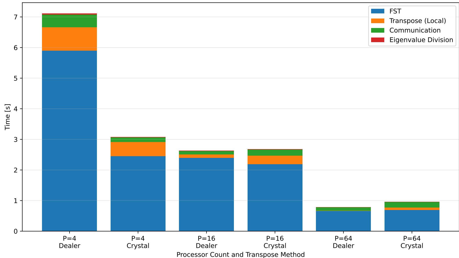
Poisson Solver Timing Breakdown, N = 8192
