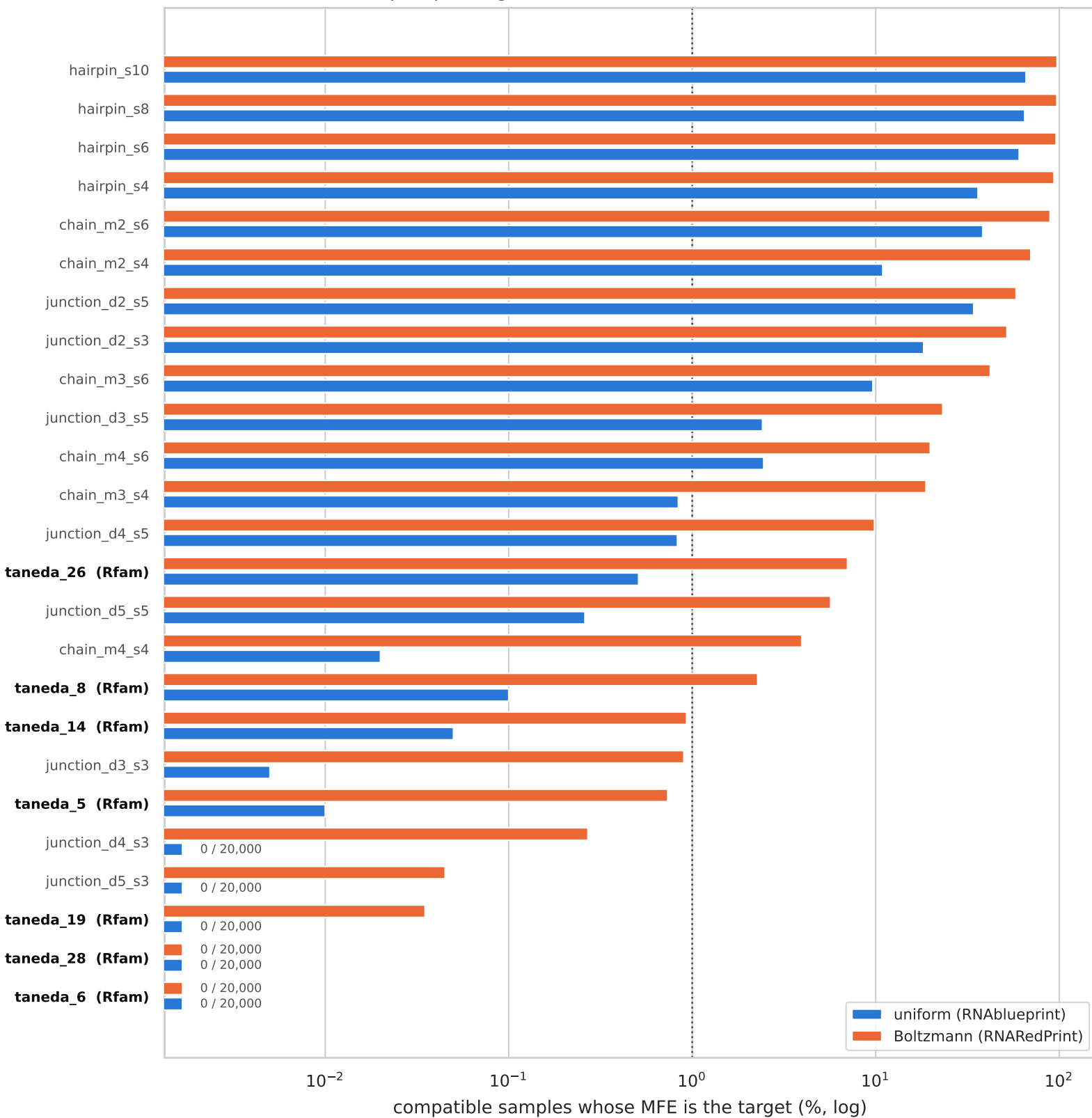
Compatible-set sampling collapses as targets get harder ViennaRNA, 20,000 samples per target; bold labels are real Rfam structures
