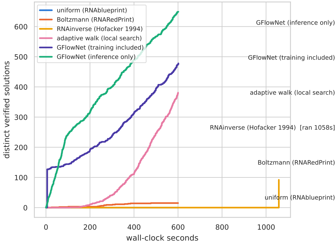
taneda_28: solutions per unit compute
