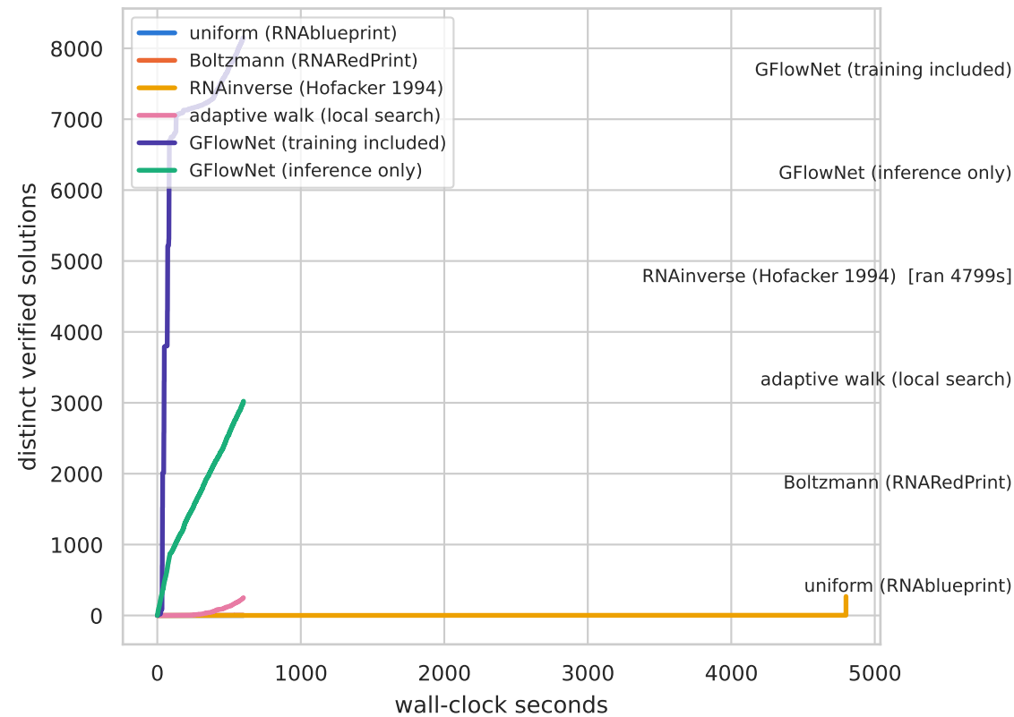
taneda_6: solutions per unit compute
