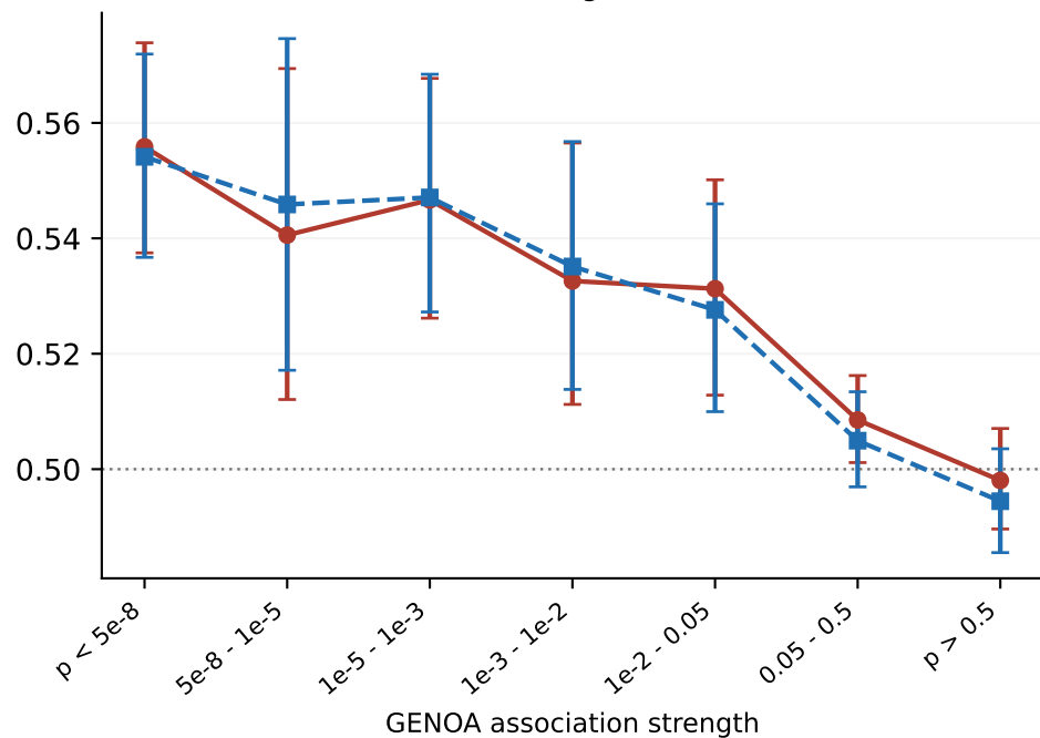
Direction agreement
