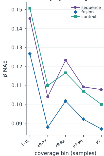
Accuracy by coverage
