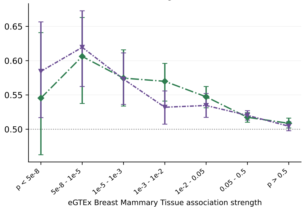
Direction agreement
