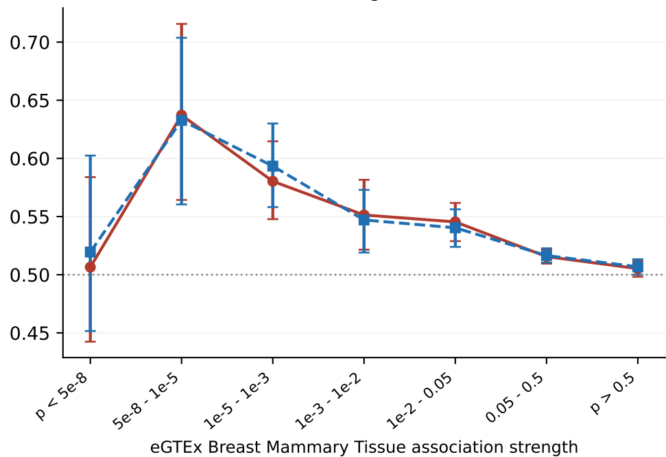
Direction agreement
