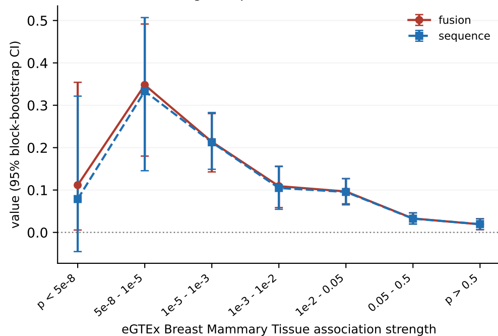
Signed Spearman correlation
